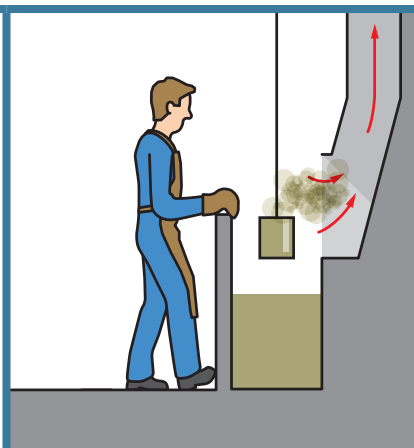
DIAGRAM 2: Side hood ventilation for an open surface tank
